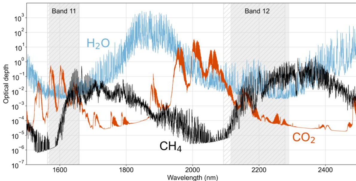
Figure 1: Methane ( \text{CH}_4 ), \text{CO}_2 , and water vapor ( \text{H}_2\text{O} ) slant optical depths in the 1500–2500 nm SWIR spectral range, based on absorption line strengths from the HITRAN database sampled at 20-pm spectral resolution. Values are for the U.S. Standard Atmosphere (Anderson et
