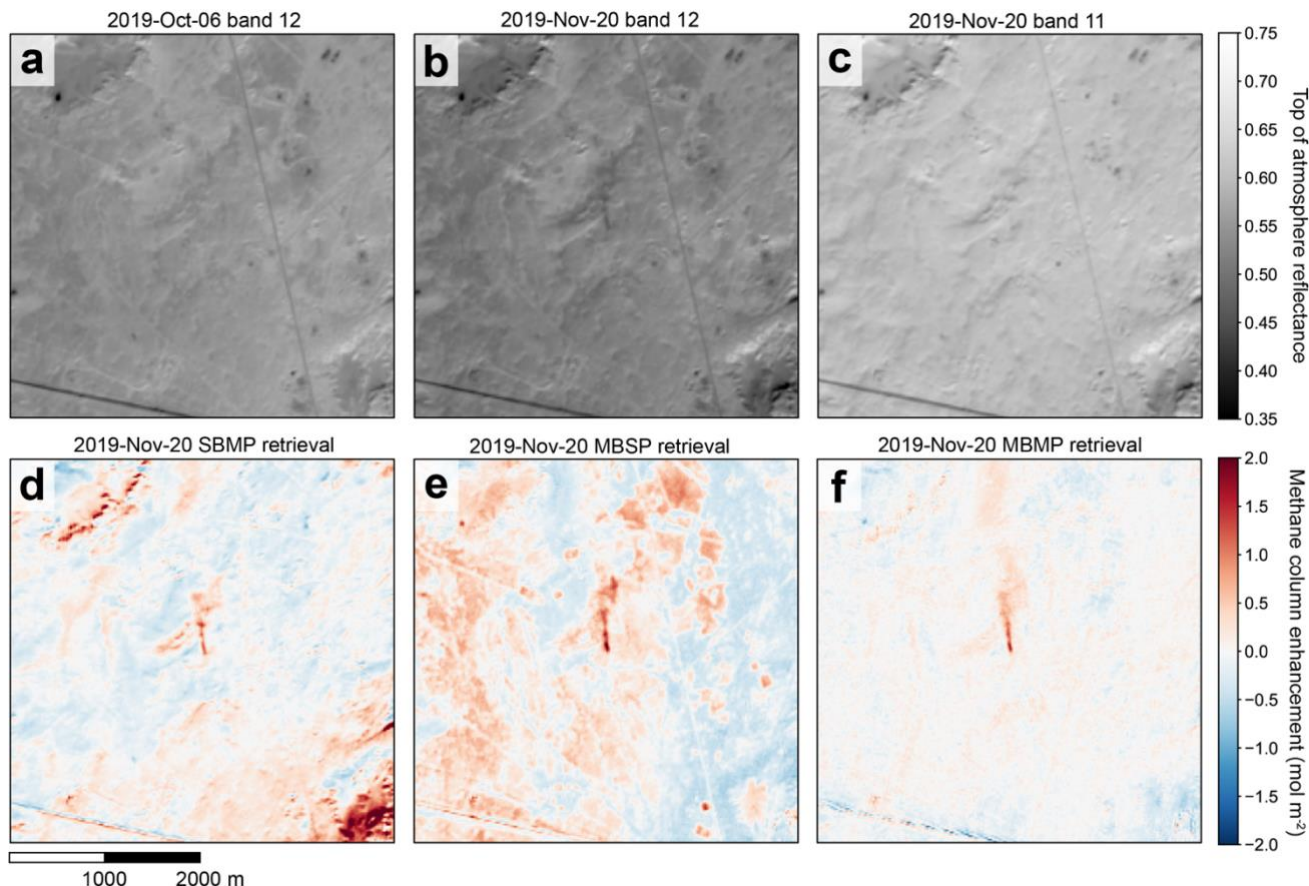
Figure 2: Demonstration of Sentinel-2 methane column retrieval for a plume emitted from a point source ( 31.6585^{\circ}\text{N} , 5.9053^{\circ}\text{E} ) in the Hassi Messaoud oil field of Algeria, on 20 November 2019 (see Section 4). (a) Sentinel-2 top of atmosphere reflectances for band-12 observed on 6 October 2019. (b) The same as panel (a), but for 20 November 2019. (c) Top of atmosphere band-11 reflectances corresponding to panel (b). (d) Single-band/multi-pass (SBMP) retrieval for 20 November 2019. (e) Multi-band/single-pass (MBSP) retrieval for 20 November 2019. (f) Multi-band/multi-pass (MBMP) retrieval for 20 November 2019.
