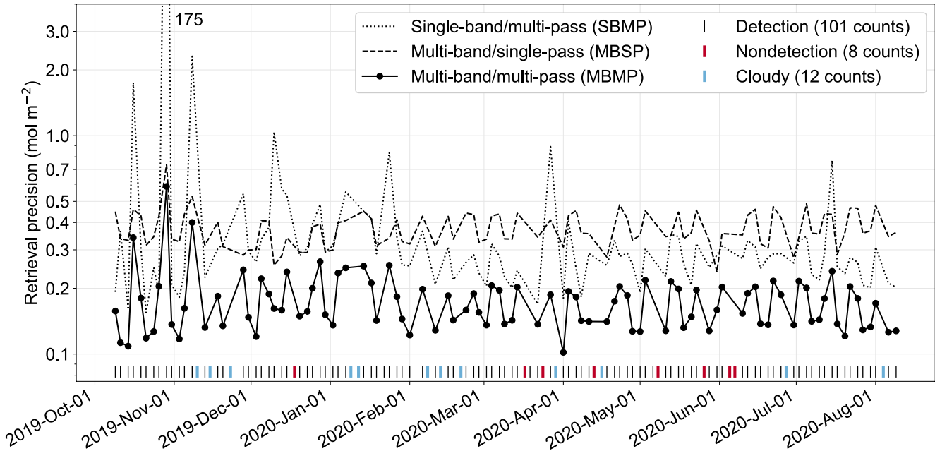
305 Figure 5: Single-pixel retrieval precision for the Hassi Messaoud scene over time, evaluated from the standard deviation of non-plume enhancements retrieved across the scene. The black, red, and blue markers indicate which satellite passes had plume detections, which had non-detections, and which were obscured by clouds, respectively. The y-axis is logarithmic.
